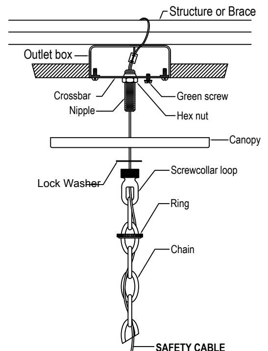
Mounting Parts
