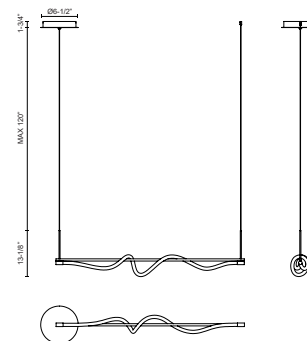
Adjustable Side Canopy Option
